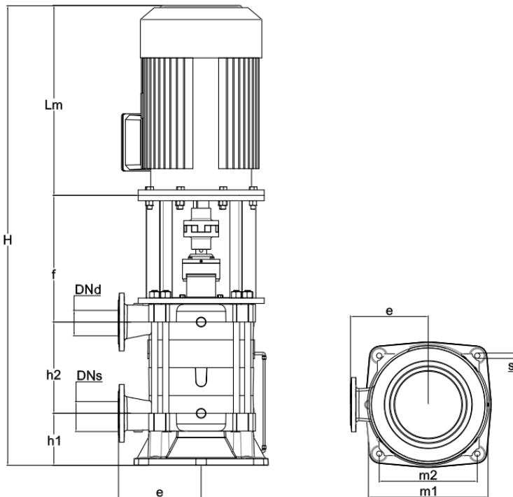
"Lm" dimension according to motor power
