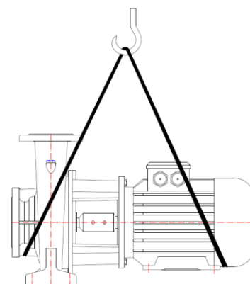
Figure 2: Transport of Pump Group
