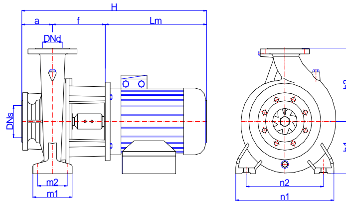
Figure 6: NMM Pump Dimensions Figure
