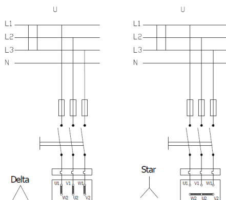
Figure 5: Electric Connection Diagram
