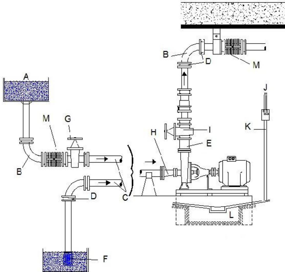
Figure 7: Sample Plumbing
