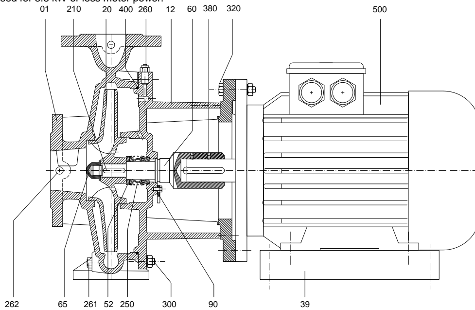
Figure 8: NMM Sectional Drawing (Without Coupling)
