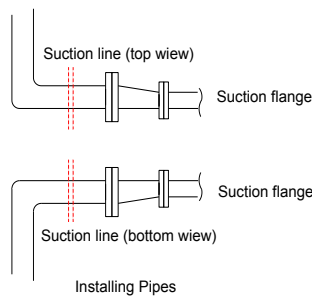
Figure 4: Piping System
