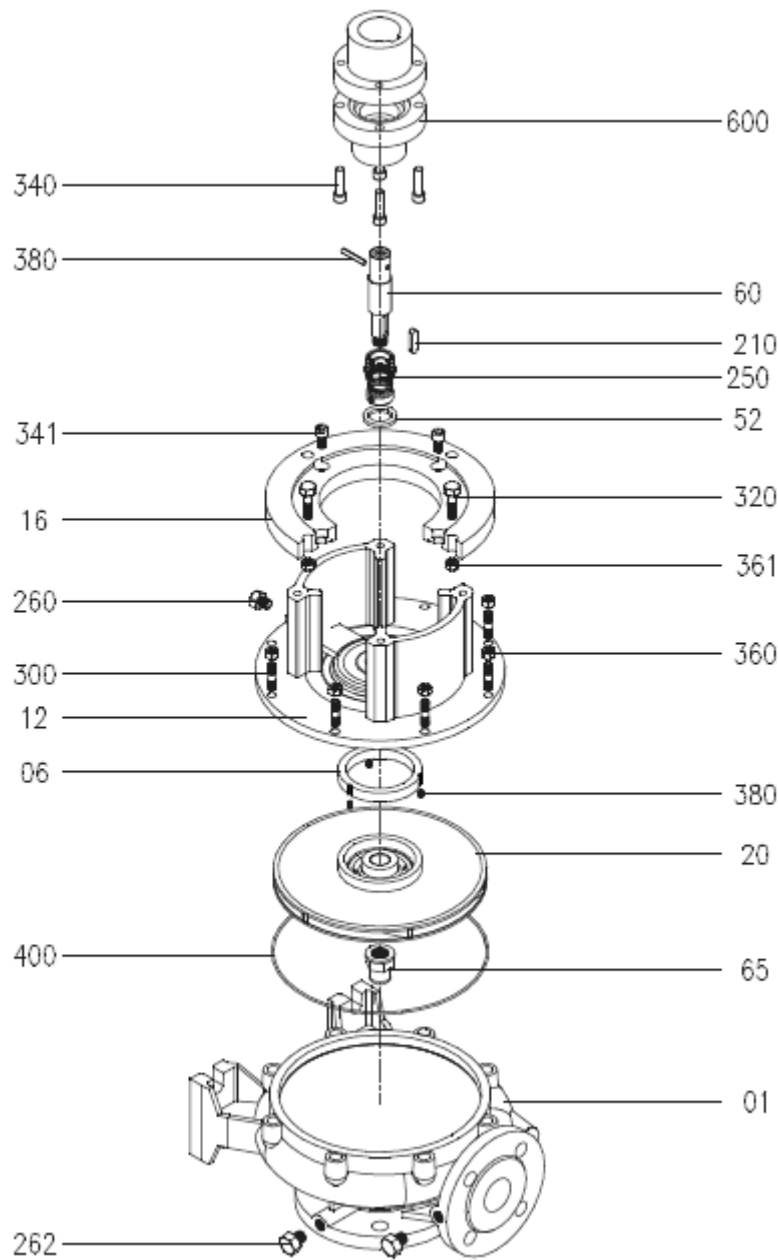
Figure 11: NMM Drawing For Dismantling (With Coupling)
