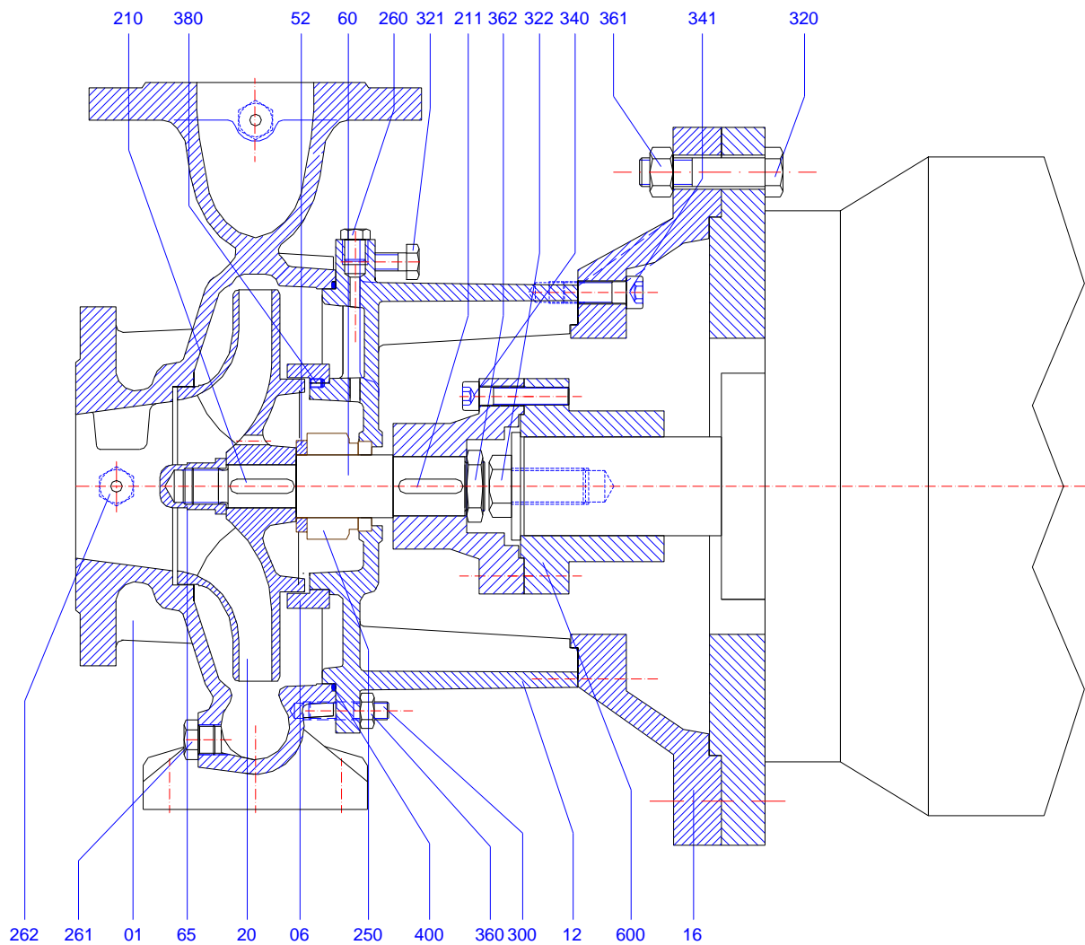
Figure 9: NMM Sectional Drawing (With Coupling)
