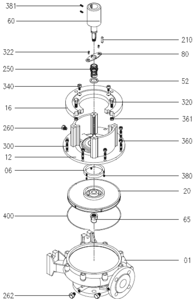
Figure 10: NMM Drawing For Dismantling (Without Coupling)
